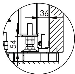
DETAIL G SCALE 2 : 15
