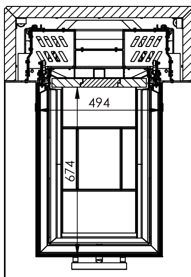
SECTION C-C SCALE 1 : 15
