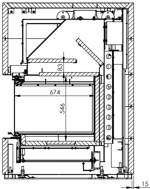
SECTION E-E SCALE 1 : 15
