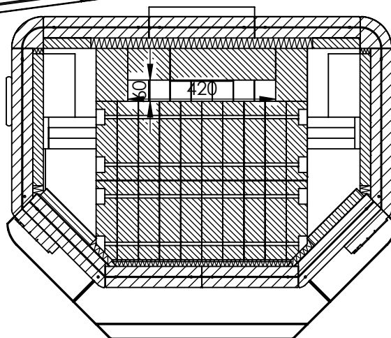
SECTION 8-8 SCALE 1 : 15
