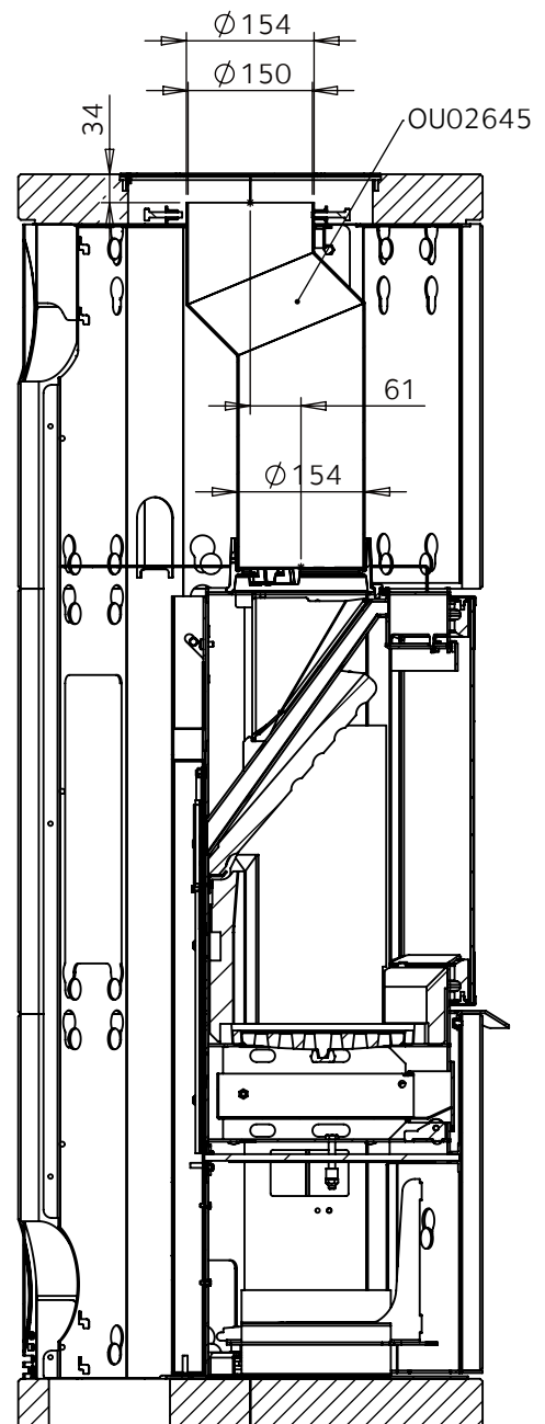
SECTION M-M SCALE 1 : 10
