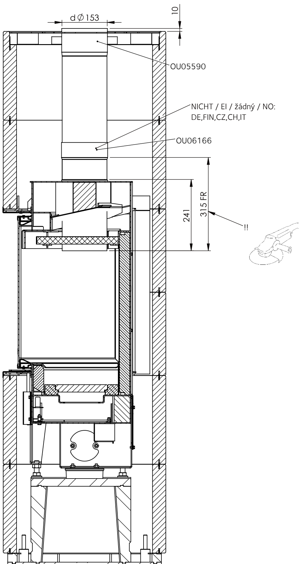
SECTION U-U SCALE 1 : 8
