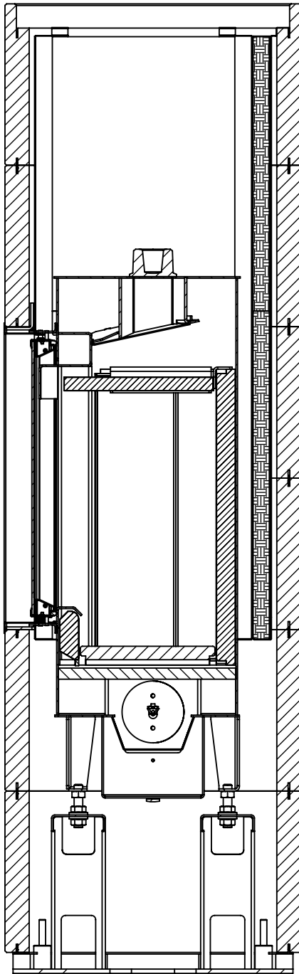
SECTION AF-AF SCALE 1 : 10
