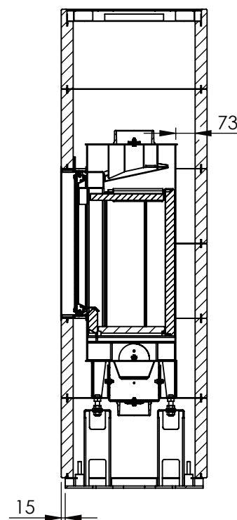
SECTION S-S SCALE 1 : 20
