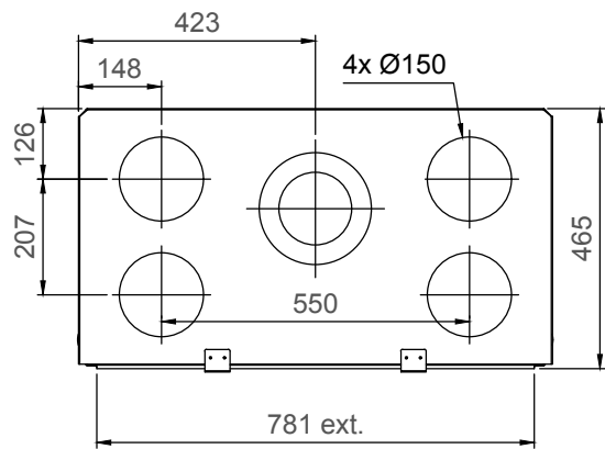
True Vision 850V - Diamond - TV - Type 1 - Coverframe
